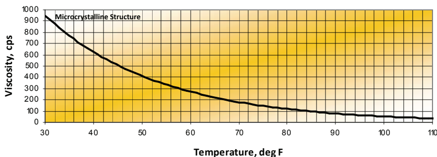
Honeybee 150 Viscosity vs Temperature
