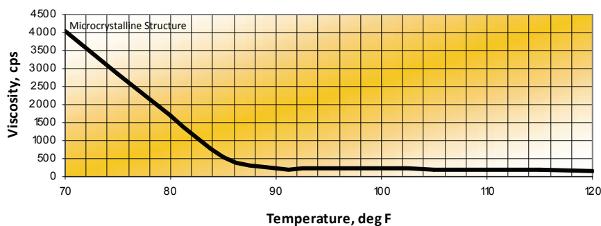
Honey Bee 230M Viscosity vs Temperature
